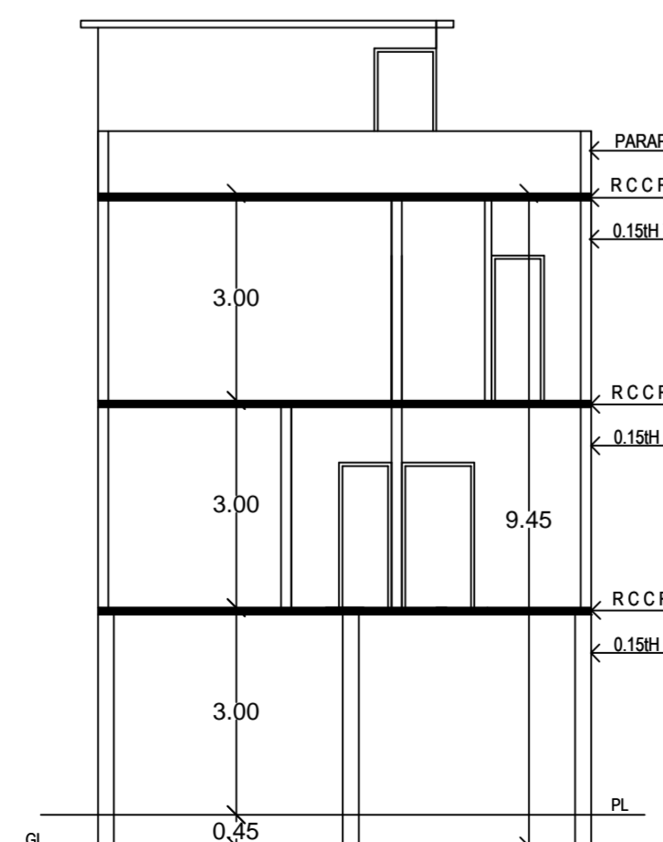
SECTION @ X-X
